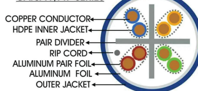
CAT6A F/FTP SERIES
